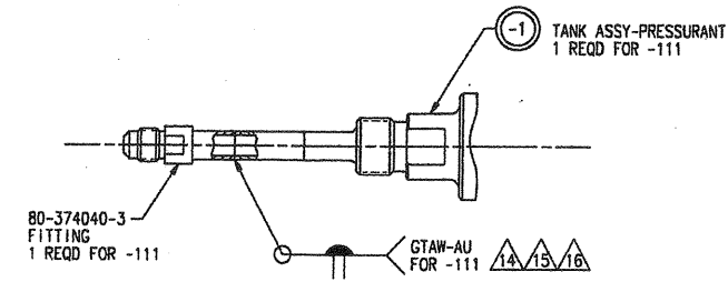
VIEW B FOR -111
