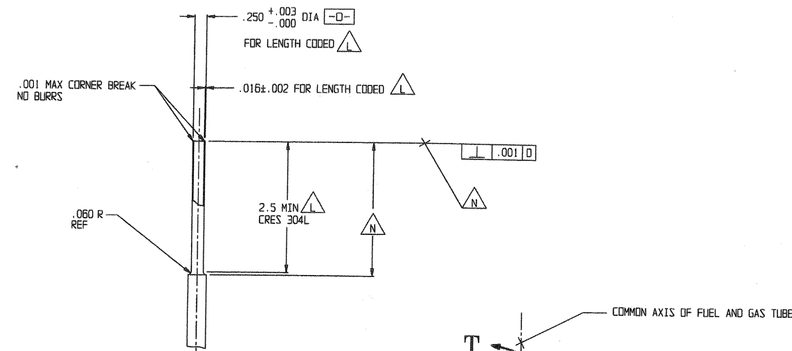
VIEW T FOR -1 SCALE 1/1
