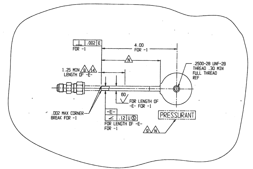
VIEW B-B SHEET 1
