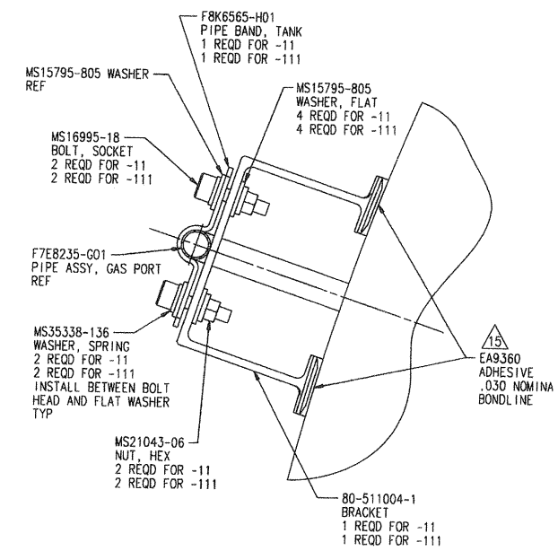
VIEW V-V PARTIAL BACKGROUND OMITTED FOR CLARITY SCALE: 2/1
