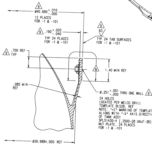
SECTION J-J SCALE: 1/1 BACKGROUND GEOMETRY OMITTED FOR CLARITY
