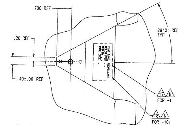
VIEW U SHEET 1
